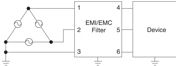
(1) Three phase (Delta-connection)
