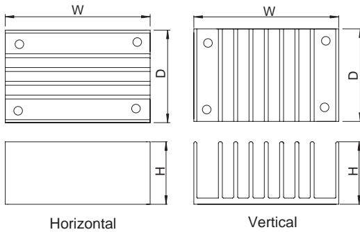
Fig.6.3 Heat Sink Types
