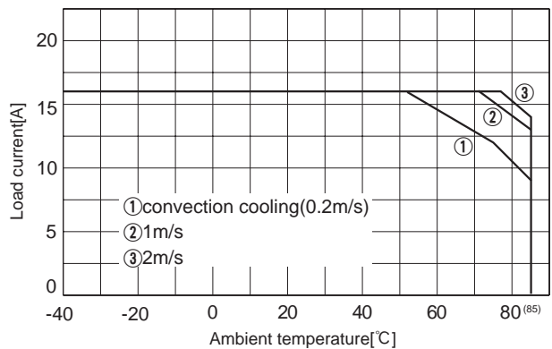
Fig.8.12 Load current vs. ambient temperature(CES48050-16 Vin=48V)
