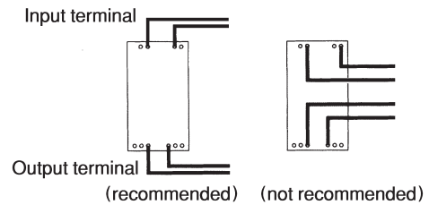
Fig.5.1 Pattern lay out
