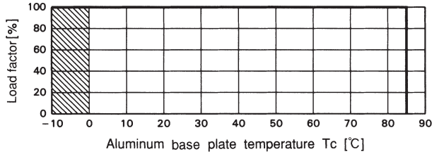
Fig.5.3 Derating curve
